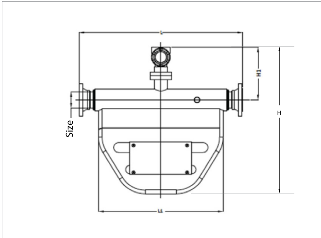
Standard Sensor (Size ½" to 8")
